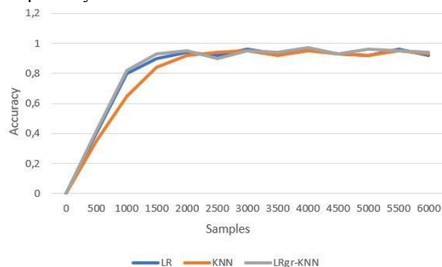
Fig. 1. Accuracy of used algorithms
