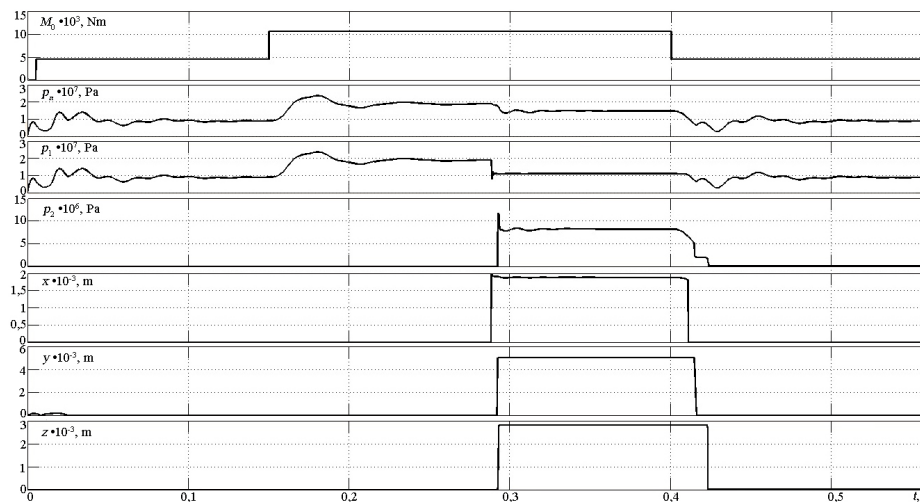
Figure 4. Theoretical graphs of transient processes of M_0(t) , p_n(t) , p_1(t) , p_2(t) , x(t) , y(t) , z(t) change.
