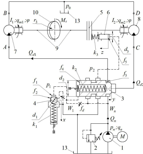
Figure 1. Calculation scheme of the conveyor hydraulic drive without taking into account elastic-inertia characteristics of its transporting part.
