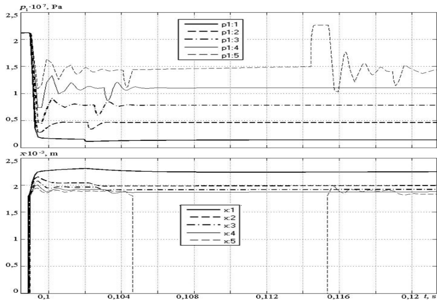
Figure 7. Theoretical graph of p_1(t) and x(t) change in time at S=0,1; 0,3; 0,5; 0,7; 0,9 .
