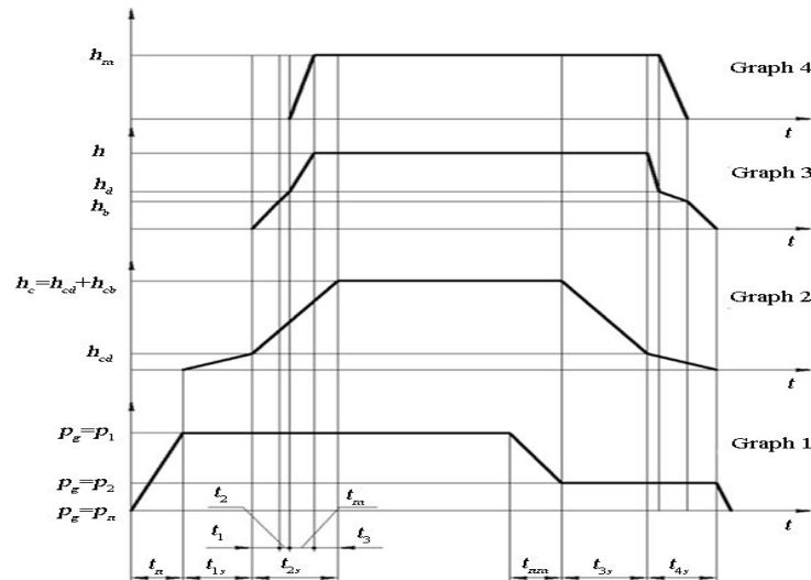
Figure 3. Sequence diagram of the conveyor adaptive hydraulic drive control system.
