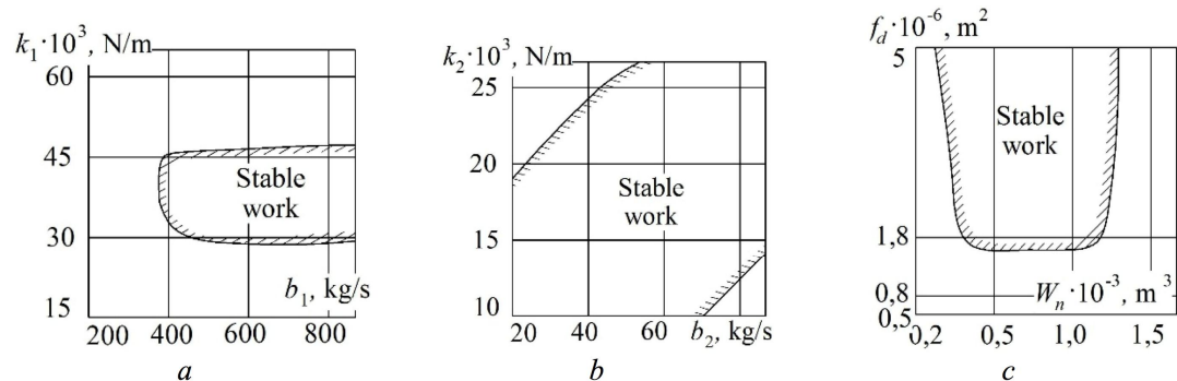
Figure 5. The impact of the parameters of the conveyor adaptive drive on the stability of its operation: a – rigidities of spring k_1 and damping factor b_1 for the sensor; b – rigidities of spring k_2 and damping factor b_2 for the distribution valve; c – area f_d of the working window of the throttle valve and the volume of hydraulic supply line W_n .
