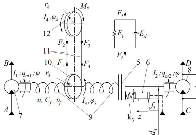
Figure 2. Calculation scheme of the transporting part of belt conveyor drive.
