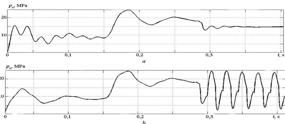
Figure 6. Theoretical graphs of pressure p_n change in time in the hydraulic supply line of the control system of the conveyor adaptive drive: a) q_{m2} \leq 0,5q_{m1} , b) q_{m2} = 0,75q_{m1} .
