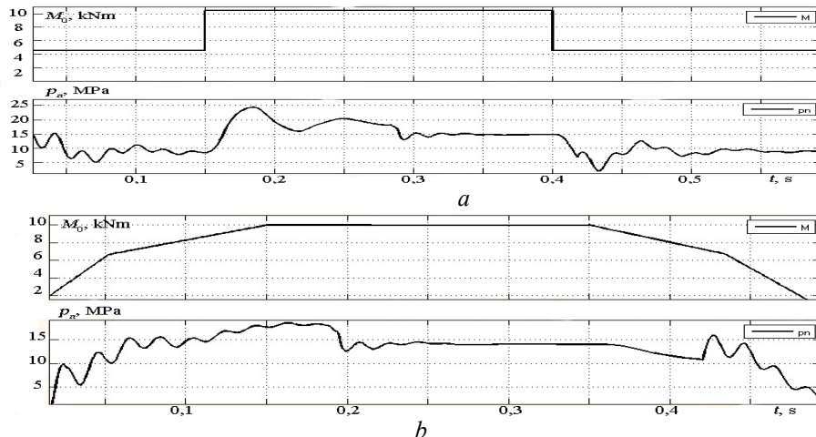
Figure 8. Theoretical graphs of load M(t) and pressure p_n(t) change character in hydraulic supply line: a – stepwise load change; b – trapezoidal load change.
