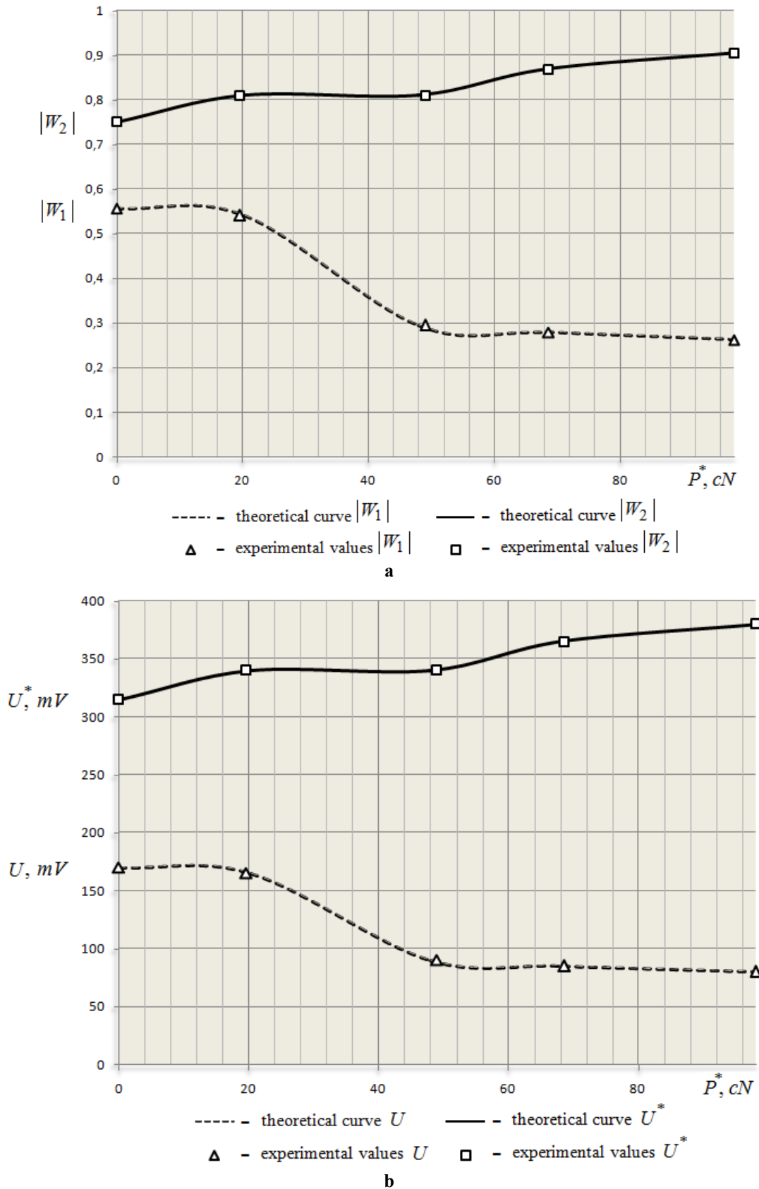
Figure 4. Dependencies of amplitude parameters on the thread tension in the waveguide: a – dependencies of amplitude parameters |W_1| , |W_2| waves on the thread tension P^* ; б – dependencies of the amplitude voltages parameters U_i , U_i^* on the thread tension P^*
