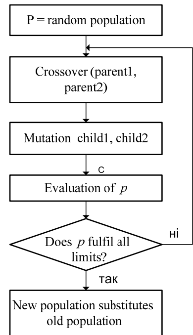
Fig.4. The genetic algorithm structure
