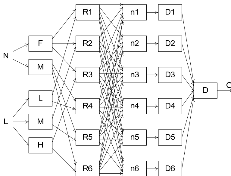
Fig. 3. The neuro-fuzzy controller block diagram
