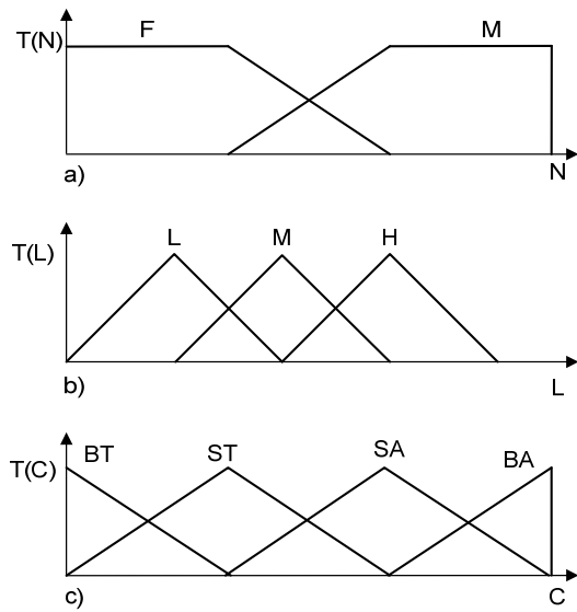
Fig.2. Membership functions for the linguistic variables
