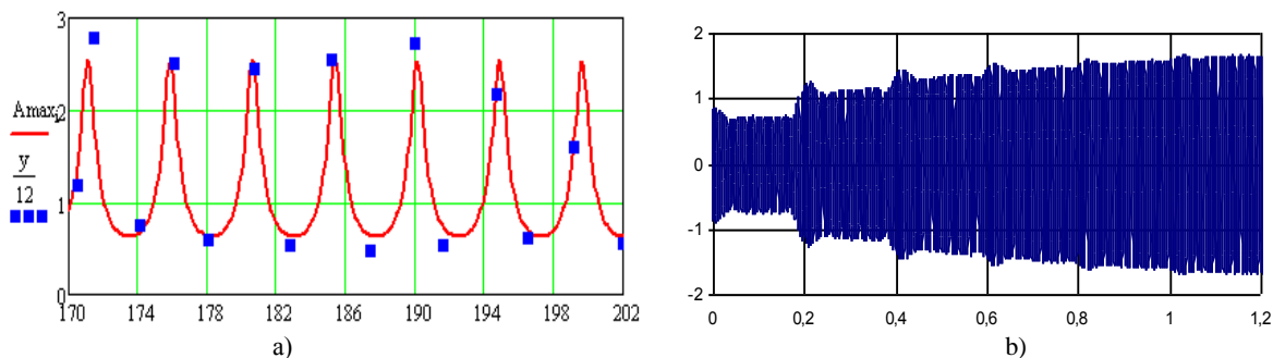
Fig. 2. a) The dependence of the amplitude of the signal on the receiver for the frequencies of the signal 170-205 kHz; b) Experimental dependence of the amplitude increase of the signal on the receiver at a frequency of 171,428 kHz
