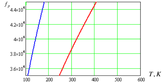
Fig. 6. Dependence of the resonant frequency on the temperature for different values of n
