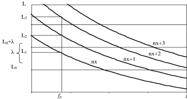
Fig. 5. Dependence of thickness on resonance frequency for different values of n
