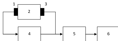
Fig. 4. Structural diagram of ultrasonic autogenerator thickness meter
