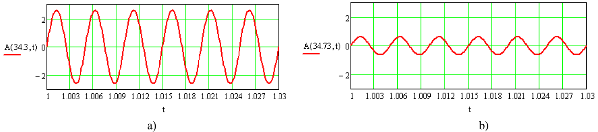
Fig. 1. Timing diagram of the signal on the receiver for the condition of resonance (a) and antiresonance (b)
