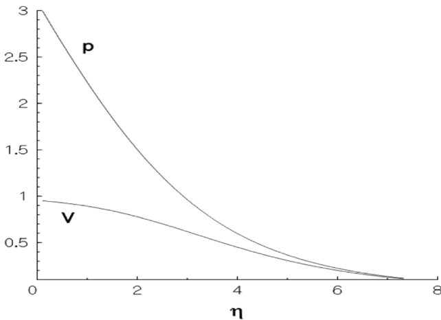
Figure 2 – The dependence of velocity and pressure values on the self-similar variable
