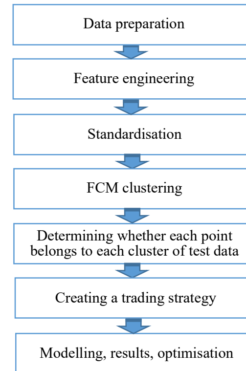
Fig. 2. Stages of the proposed methodological approach
