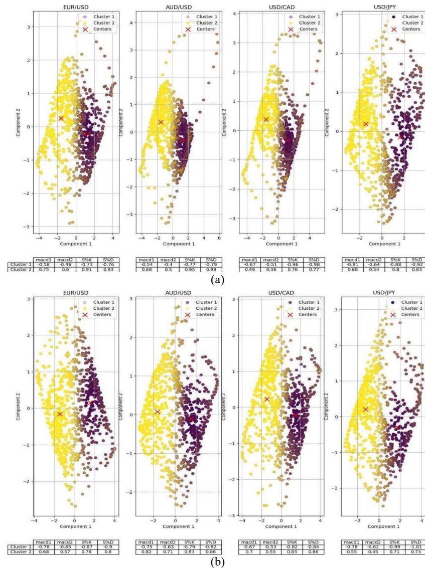
Fig. 7. Two-dimensional PCA representation of FCM clustering on training samples of four currency pairs for daily (a) and four-hour (b) timeframes
