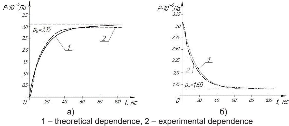
Fig. 1. The diagram of change of force loading of muscular fabric in the modes: a) isometric tetanus; б) muscle relaxation at a constant rate
