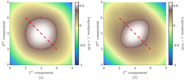
Figure 7: Modified Lagrangian, \mathcal{J}^*(\mathbf{y}^{(i)}, \zeta) , \zeta = 0.05 : (a) Gaussian noise, \sigma = 2.5 ; (b) Laplacian noise, b = 2.5 .
