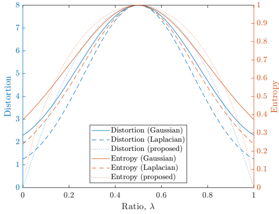
Figure 10: Distortion and entropy plots for Gaussian, Laplacian, and the proposed obfuscation models defined for the line segment \mathbf{X}_{i,R}\mathbf{X}_{i,B} .
