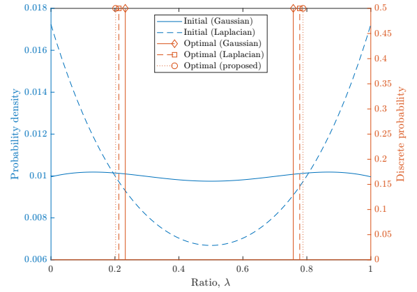
Figure 12: Continuous and discrete densities, \phi_{\mathbf{Y}_i}^l , for mixtures produced by obfuscation methods on \mathbf{X}_{i,R}\mathbf{X}_{i,B} .
