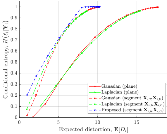
Figure 13: Plots for obfuscation efficiency.
