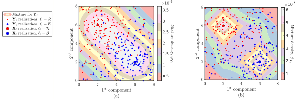
Figure 4: Mixtures \phi_{Y_i} resulting from addition of bi-variate independent noise to \mathbf{X}_{i,R} and \mathbf{X}_{i,B} : (a) Gaussian noise, \sigma = 2.5 ; (b) Laplacian noise, b = 2.5 .
