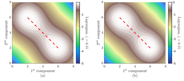
Figure 9: Modified Lagrangian, \mathcal{J}^*(\mathbf{y}^{(i)}, \zeta) , \zeta = 0.15 : (a) Gaussian noise, \sigma = 2.5 ; (b) Laplacian noise, b = 2.5 .
