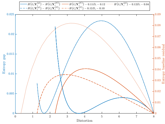
Figure 11: Residual performance plots for Gaussian, Laplacian, and the proposed obfuscation models defined for the line segment \mathbf{X}_{i,R}\mathbf{X}_{i,B} .
