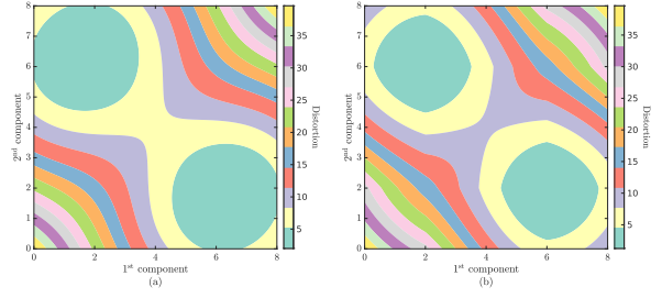
Figure 5: For every \mathbf{y}^{(i)} on the plane, distortion is D_i(\mathbf{y}^{(i)}) = d(\mathbf{y}^{(i)}, \mathbf{X}_{i,R})\Pr(\ell_i = \mathcal{R}|\mathbf{y}^{(i)}) + d(\mathbf{y}^{(i)}, \mathbf{X}_{i,B})\Pr(\ell_i = \mathcal{B}|\mathbf{y}^{(i)}) : (a) Gaussian noise, \sigma = 2.5 ; (b) Laplacian noise, b = 2.5 .
