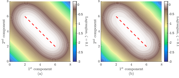
Figure 8: Modified Lagrangian, \mathcal{J}^*(\mathbf{y}^{(i)}, \zeta) , \zeta = 0.1 : (a) Gaussian noise, \sigma = 2.5 ; (b) Laplacian noise, b = 2.5 .
