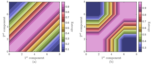
Figure 6: Entropy of inference, H(\ell_i|\mathbf{Y}_i = \mathbf{y}^{(i)}) , for different realizations of \mathbf{Y}_i : (a) Gaussian noise, \sigma = 2.5 , H(\ell_i|\mathbf{Y}_i) \approx 0.6 ; (b) Laplacian noise, b = 2.5 , H(\ell_i|\mathbf{Y}_i) \approx 0.6 .
