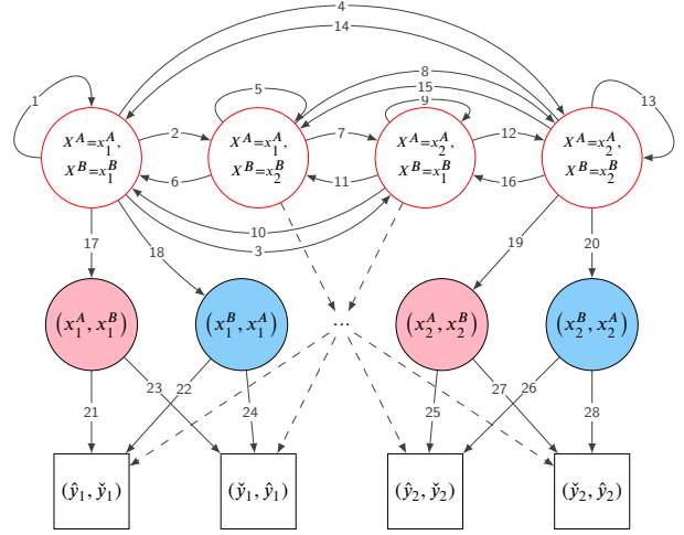
Figure 2: Hidden Markov Model for 2 users sending CAMs.
