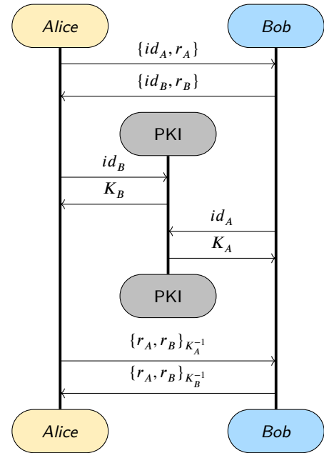
Figure 14: Protocol for mutual authentication of Alice and Bob .
