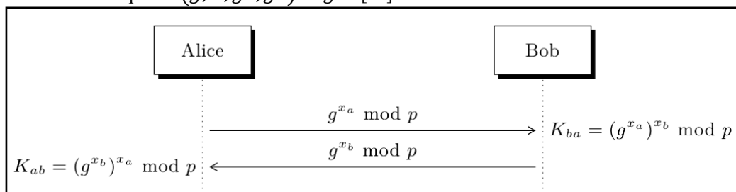
Fig.1. Diffie-Hellman protocol
